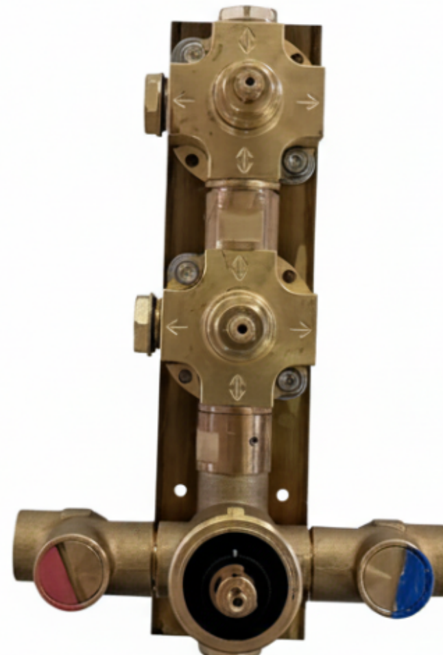
Thermostatic valve
