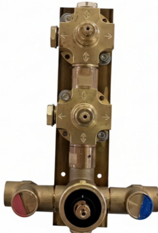
Thermostatic valve
