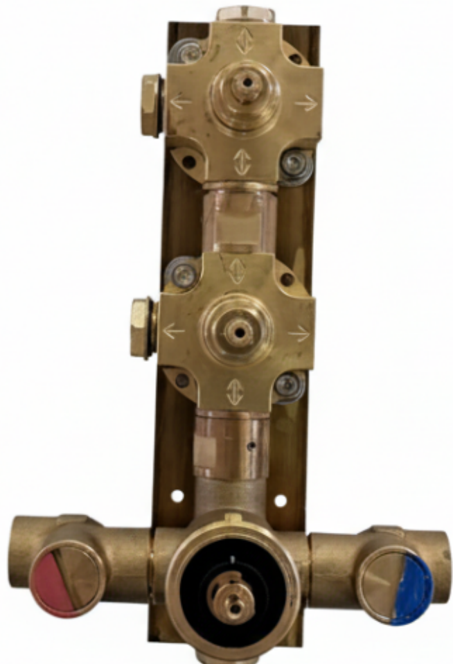
Thermostatic valve
